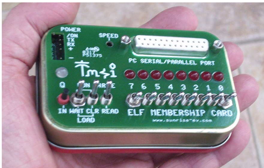
The complete package: The Membership Card, Front Panel, and Cover Card all fit in an Altoids tin.
